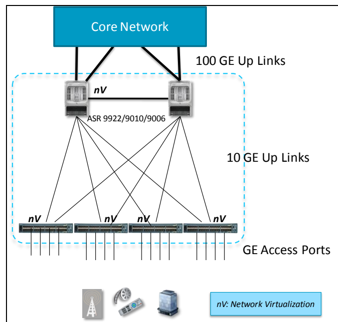
Figure 1. ASR 9000 System Network Configuration
