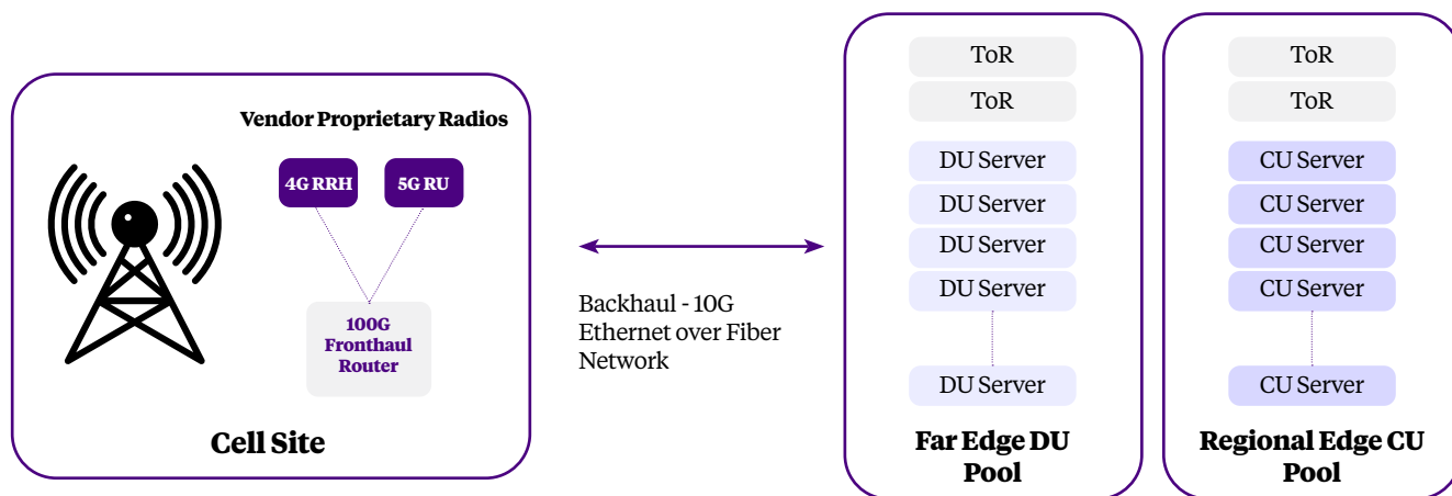
Figure 6. Open C-RAN
