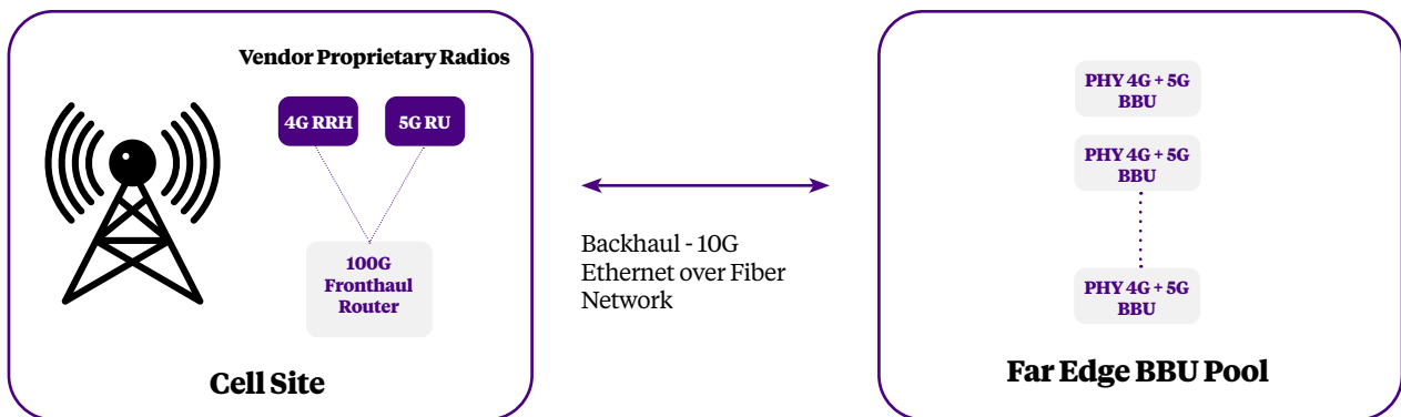
Figure 4 . PHY C-RAN
